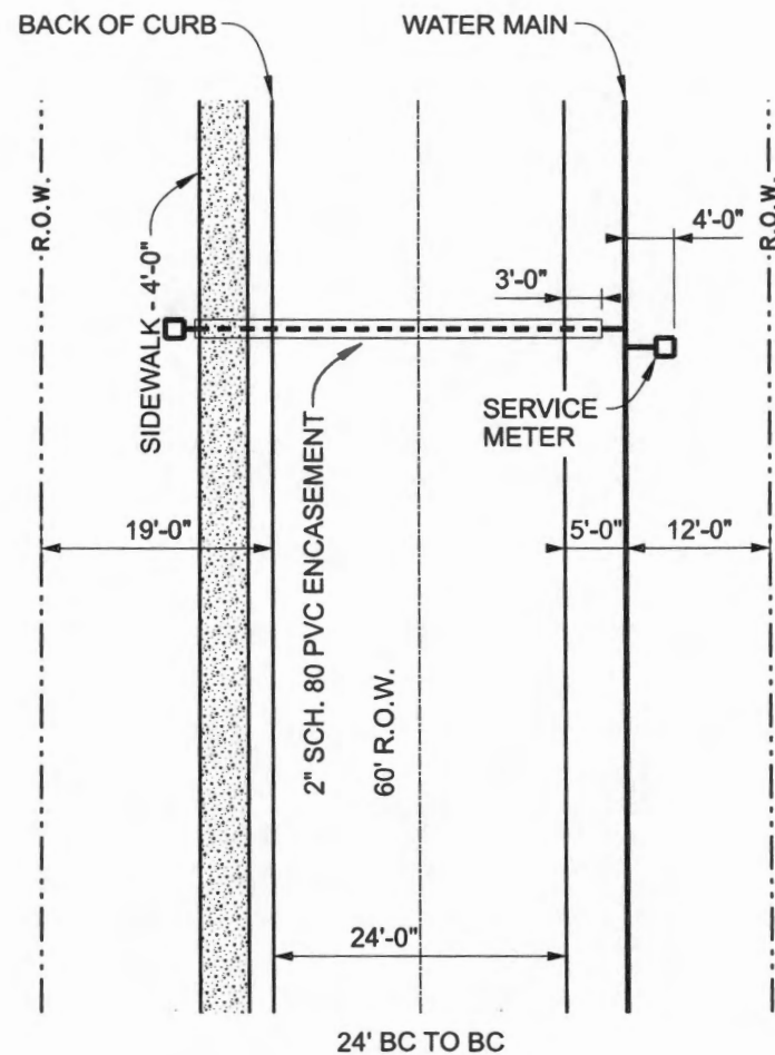
DETAIL OF METER PLACEMENT 60' R.O.W. WITH 4' SIDEWALK
