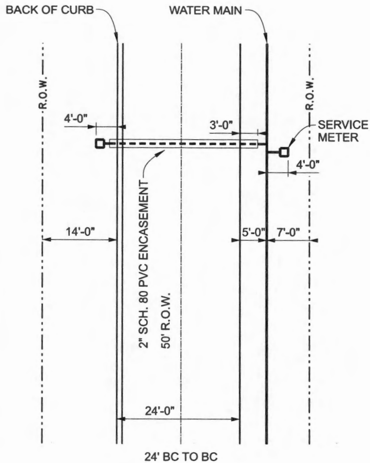
DETAIL OF METER PLACEMENT 50' R.O.W.
